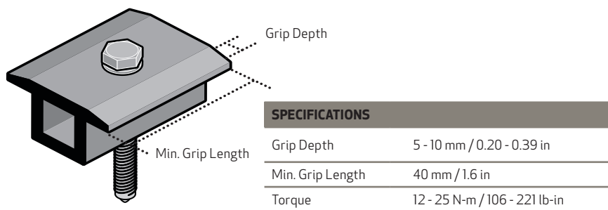
Fig. 1-1 Clamp Specifications
