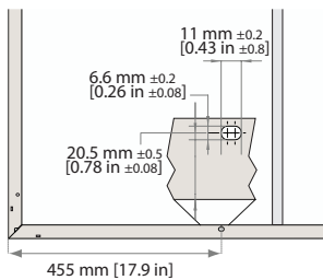
Fig. 1-3 Mounting holes: REC Alpha Panels
