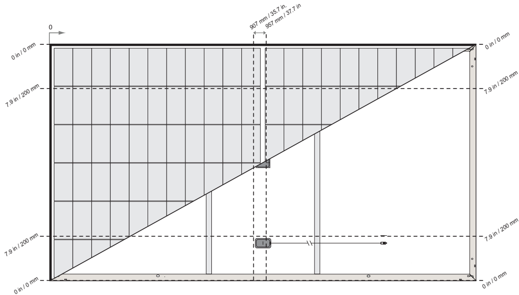
Fig. 2-5 Mixed Six-Point Mounting of REC Alpha Pure 2 Series Panels using short rails
