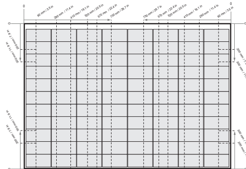
Fig. 4-1 Clamping of REC Alpha Pure-RX panels using short rails
