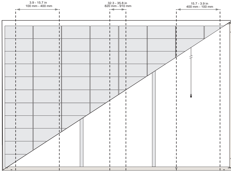
Fig. 4-2 Six-point mounting configuration clamping zones: REC Alpha Pure-RX
