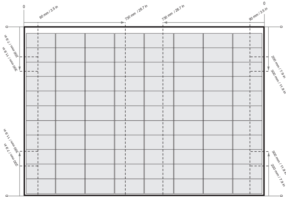
Fig. 3-4 Clamping of REC Alpha Pure-RX panels with Rails parallel to the Long Side of the Panel
