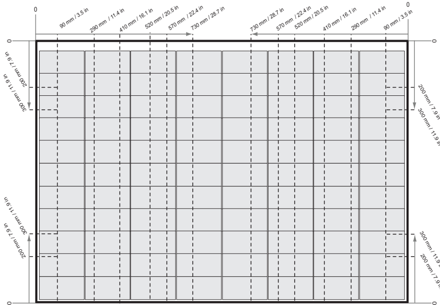
Fig. 3-3 Clamping of REC Alpha Pure-RX panels with Rails parallel to the Short Side of the Panel
