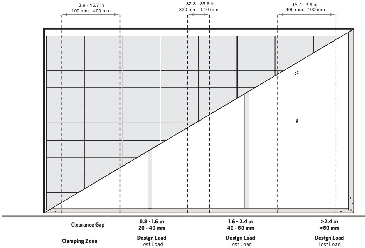
Six-point mounting configuration clamping zones: REC Alpha Pure-R
