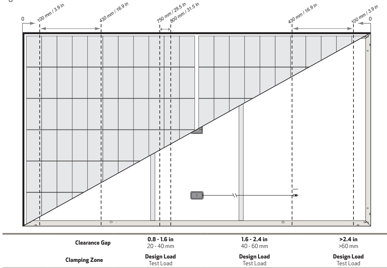
Fig. 2-4 Six-point mounting configuration clamping zones: REC Alpha Pure 2
