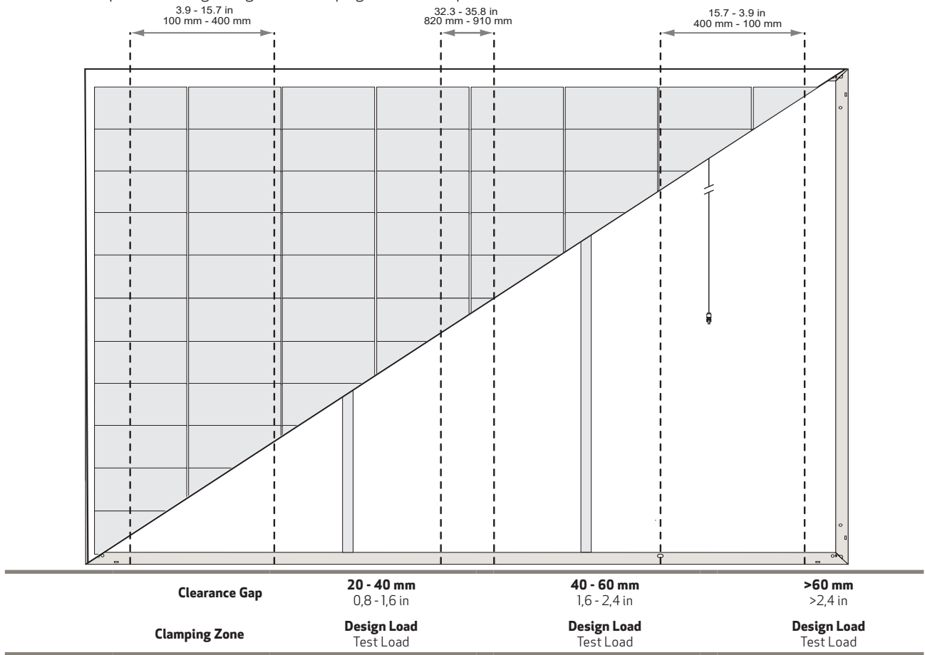
Six-point mounting configuration clamping zones: REC Alpha Pure-RX
