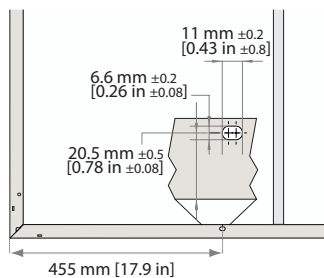
Fig. 3 Mounting holes: REC Alpha Panels
