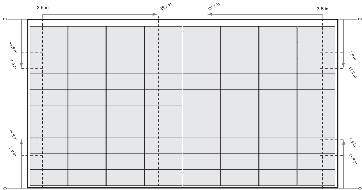
Fig. 4-2 Clamping of REC Alpha Pure-R Series panels with Rails parallel to the Long Side of the Panel
