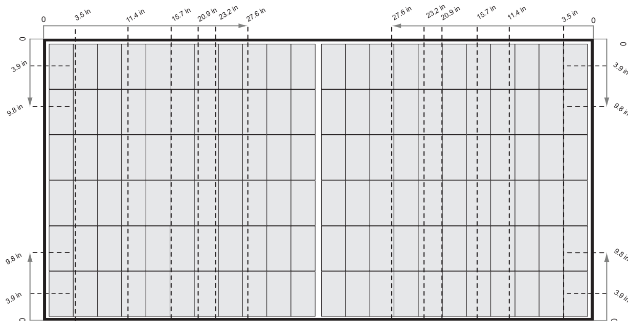
Fig. 3-1 Clamping of REC Alpha Pure 2 Series panels with Rails parallel to the Short Side of the Panel
