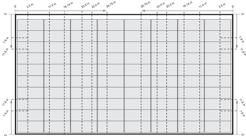
Fig. 4-1 Clamping of REC Alpha Pure-R Series panels with Rails parallel to the Short Side of the Panel
