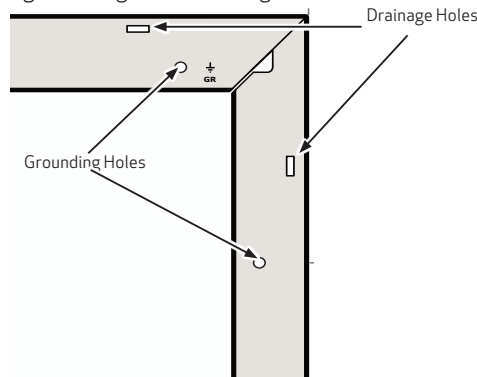
Fig. 5 Drainage and Grounding Holes
