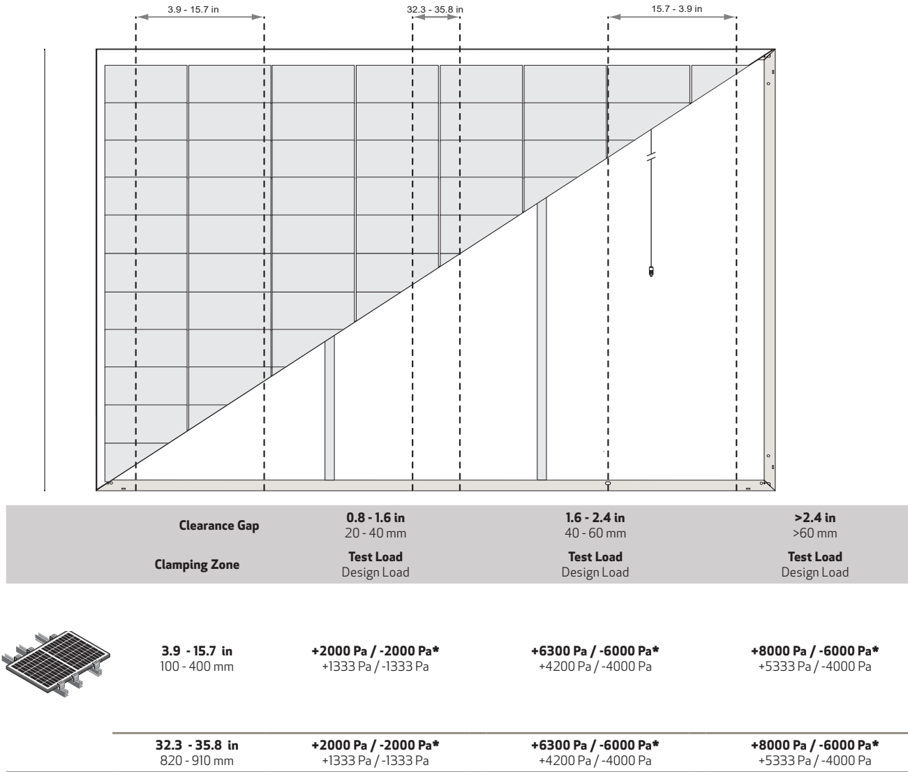
Fig. 5-4 Six-point mounting configuration clamping zones: REC Alpha Pure-RX Series
