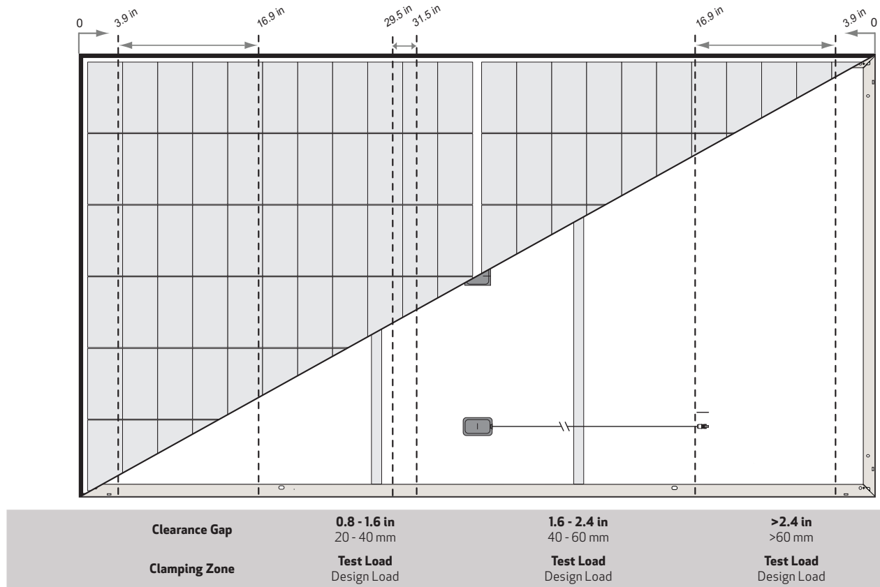
Fig. 3-4 Six-point mounting configuration clamping zones: REC Alpha Pure 2 Series
