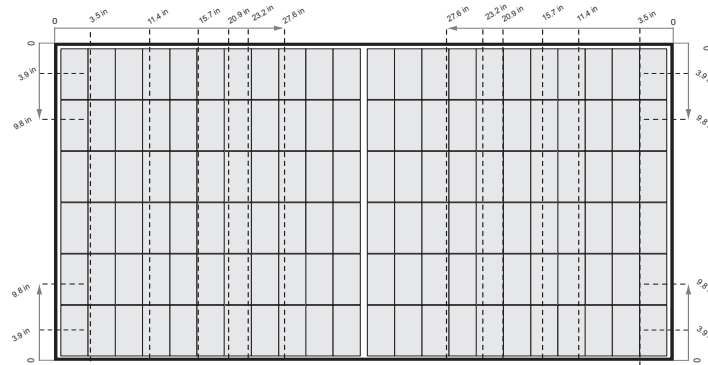
Fig. 3-3 Clamping of REC Alpha Pure 2 Series panels using short rails
