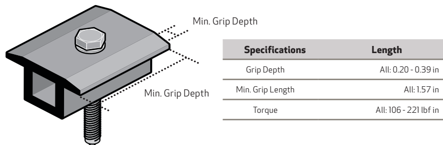
Fig. 1 Clamp Specifications
