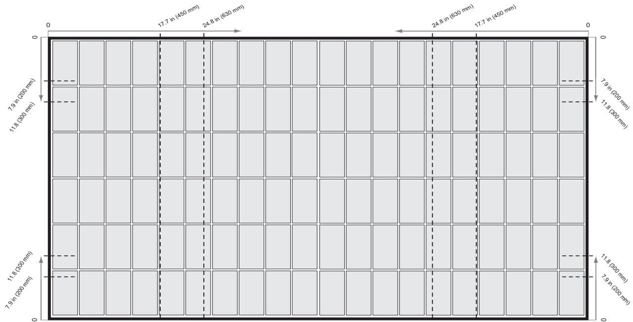
Fig. 3-2 Clamping of REC Alpha Pro MG Series panels with Rails parallel to the Long Side of the Panel
