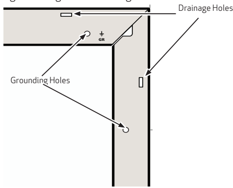
Fig. 5 Drainage and Grounding Holes
