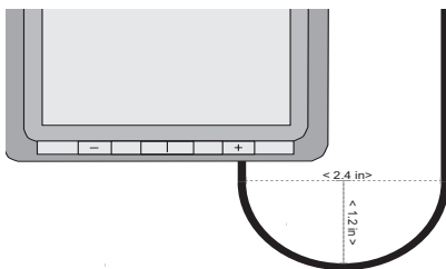
Fig. 7 Minimum Cable Distance
