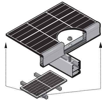
Fig. 4 Mounting hole installation example
