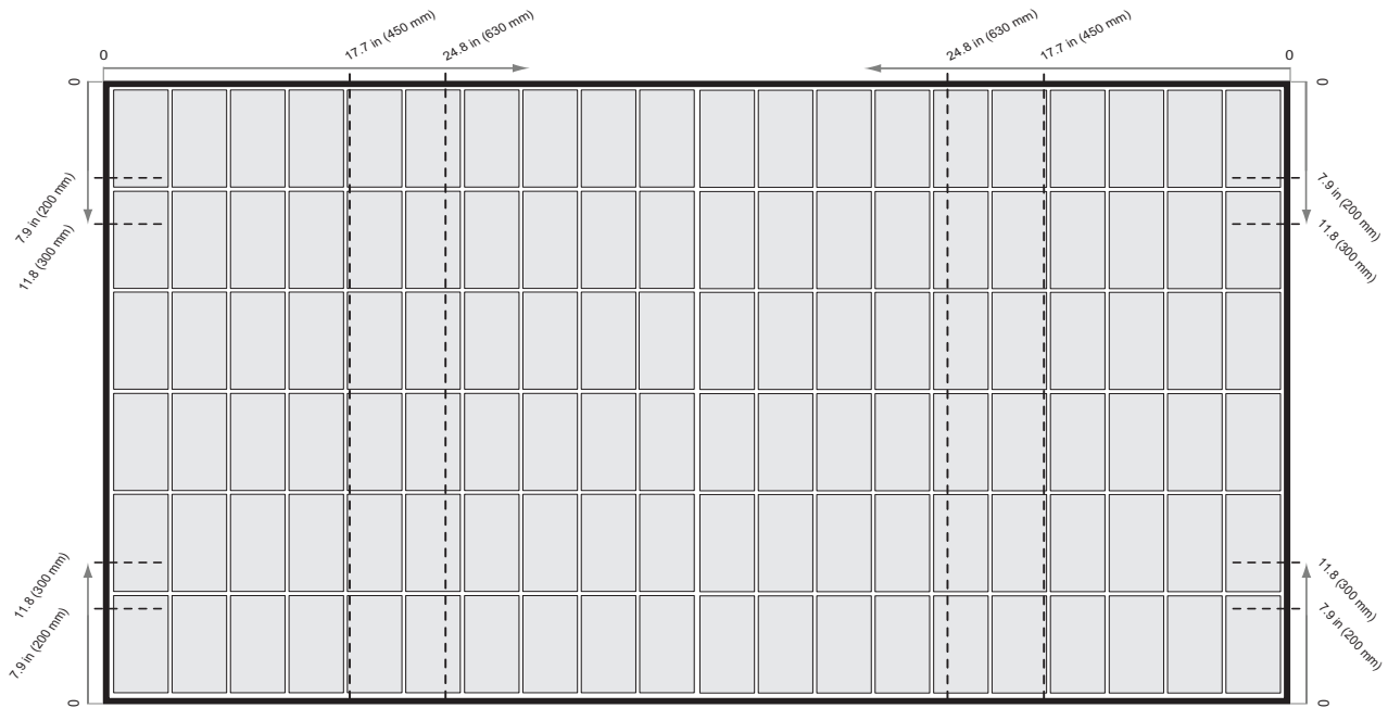
Fig. 2-2 Clamping of REC Alpha Pro M panels with Rails parallel to the Long Side of the Panel
